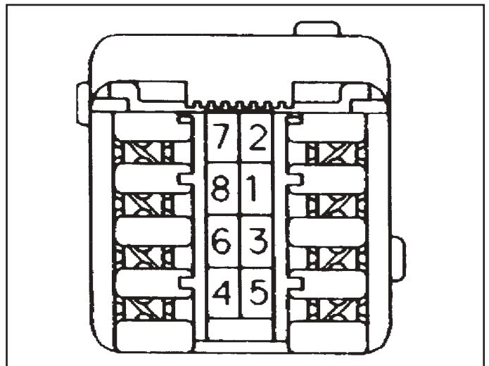
Wiring Configuration
